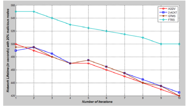
Fig. 12 Network Lifetime analysis of FTRS, AODV, 2-ACKT and GTMS against some iterations with 20% of malicious nodes
