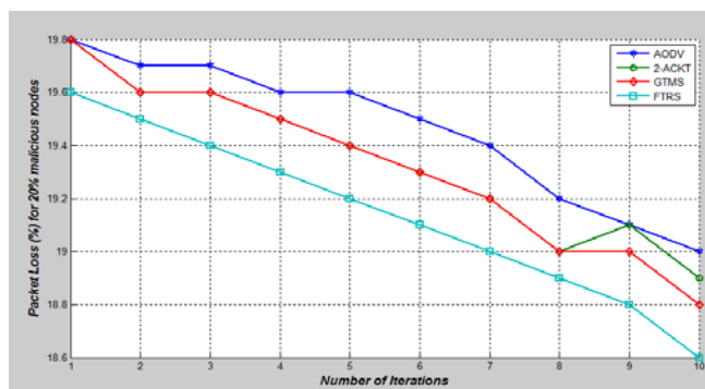
Fig. 6 Packet loss analysis of FTRS, AODV, 2-ACKT and GTMS against some iterations with 20% of malicious nodes
