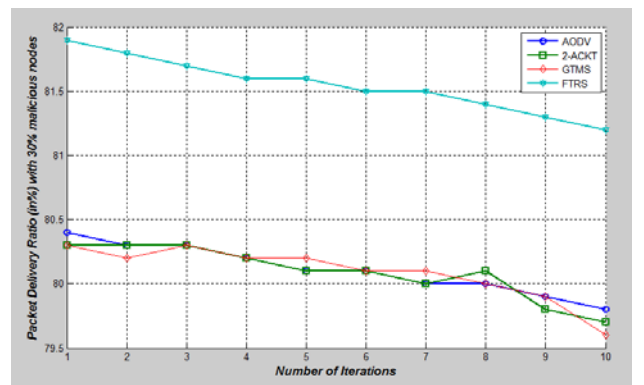
Fig. 10 Packet delivery ratio analysis of FTRS, AODV, 2-ACKT, and GTMS against some iterations with 30% of malicious nodes
