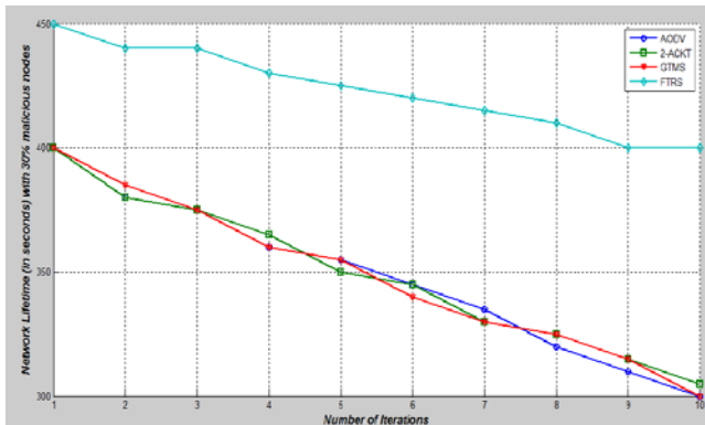
Fig. 13 Network Lifetime analysis of FTRS, AODV, 2-ACKT and GTMS against some iterations with 30% of malicious nodes
