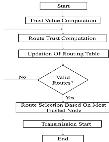
Fig. 1 Before Packet Transmission Process
