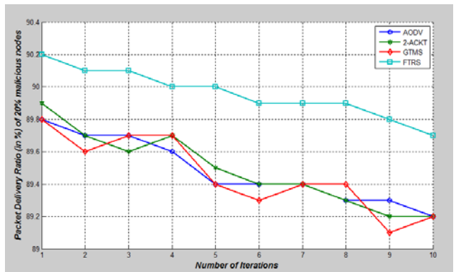
Fig. 9 Packet delivery ratio analysis of FTRS, AODV, 2-ACKT and GTMS against some iterations with 20% of malicious nodes
