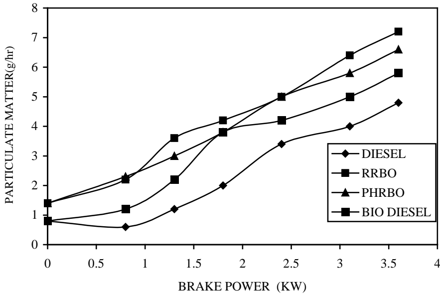
Fig .10 Variation Of Particulate Emission With Brake Power
