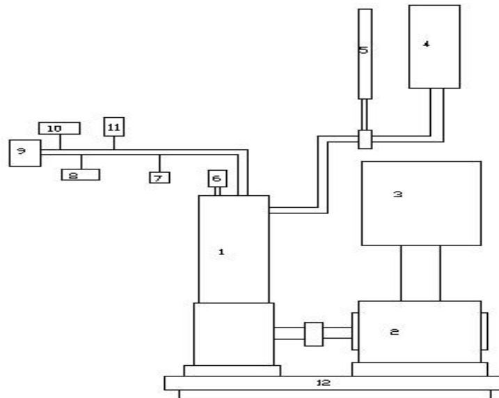
Fig. 2 Experimental set up
