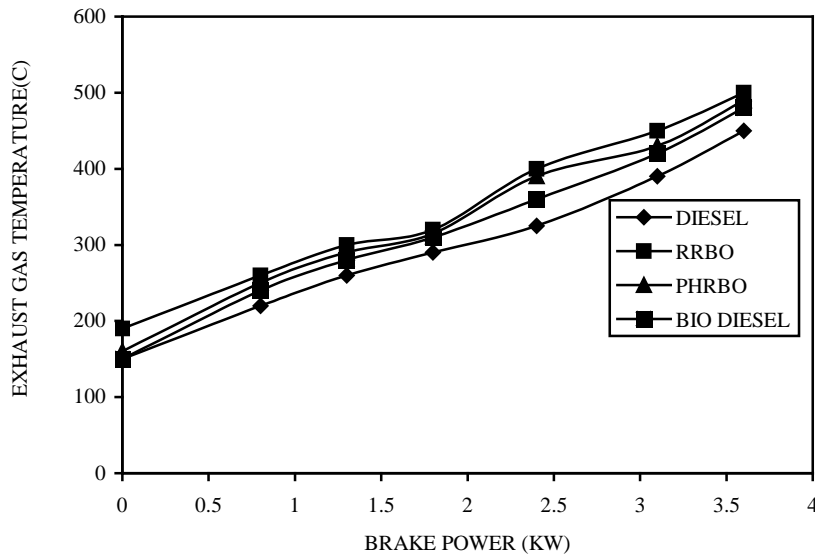
Fig 5 Variation Of Exhaust Gas Temperature With Brake Power
