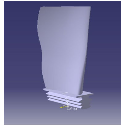
Fig. 8 The 3D shape of the Combined Blade Model
