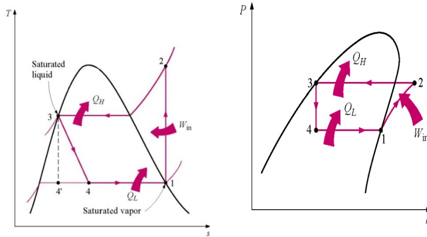
Fig. 2 T-s &amp; p-h diagram
