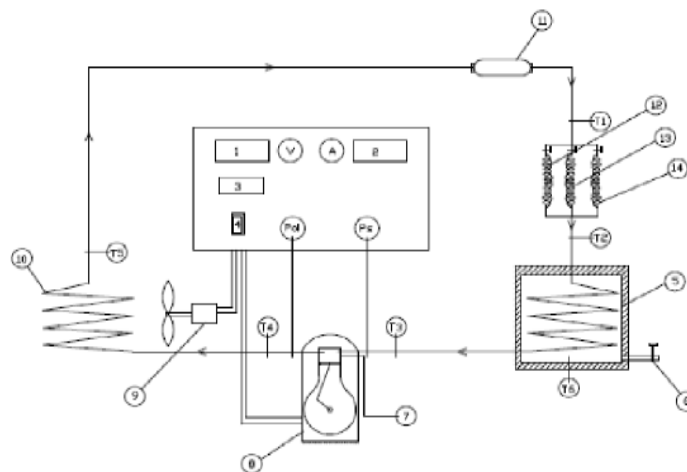
Fig Schematic diagram of experimental setup.
