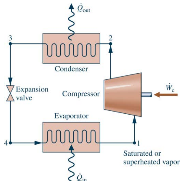
Fig.1 Vapor Compression Refrigeration System
