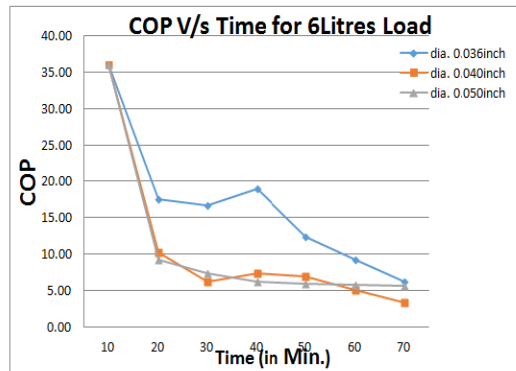
Graph 5.1.2.3 COP Vs TIME for different tube diameters & Loads
