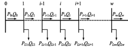
Fig. 1 Single-line diagram of a main feeder
