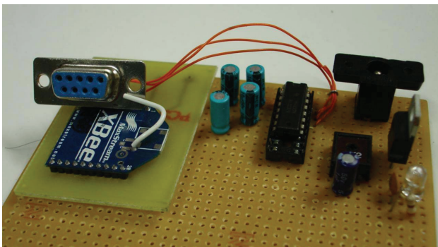
Fig. 6 Hardware structure of receiving node.
