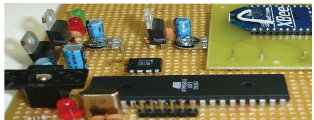
Fig.4 Hardware structure of transmitting node.
