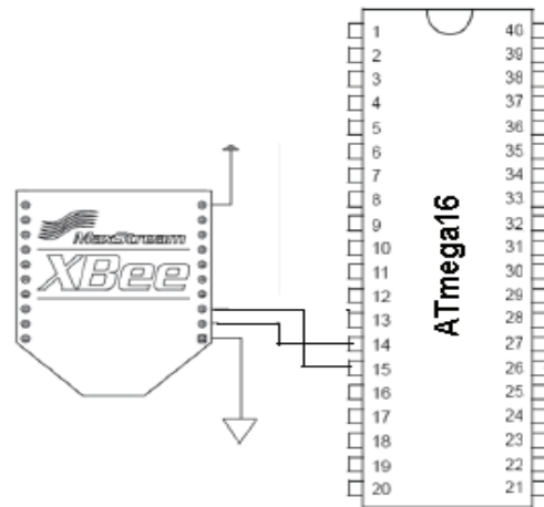
Fig. 3 Interfacing of Xbee with Microcontroller
