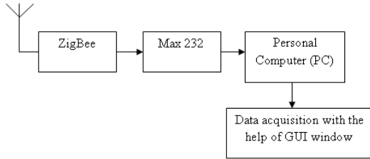
Fig. 5 Block Diagram of receiving node
