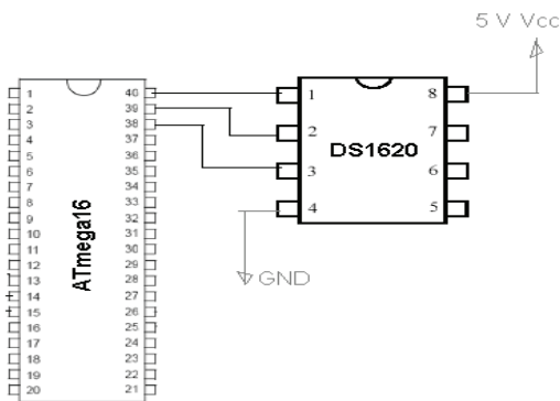
Fig. 2 Interfacing DS1620 with Microcontroller
