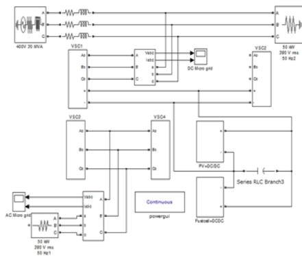
Fig. 9 Simulation of hybrid micro grid
