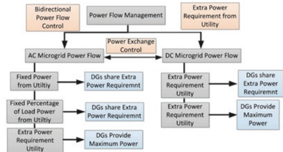
Fig. 6 Power flow management of the proposed method
