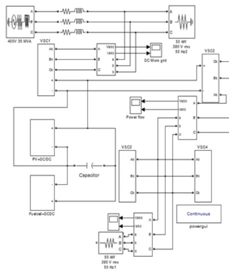
Fig. 10 Simulation of Mode 1 operation
