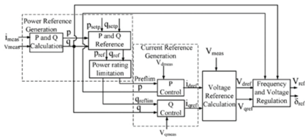
Fig. 5 Control layout of the VSC interfaces micro sources
