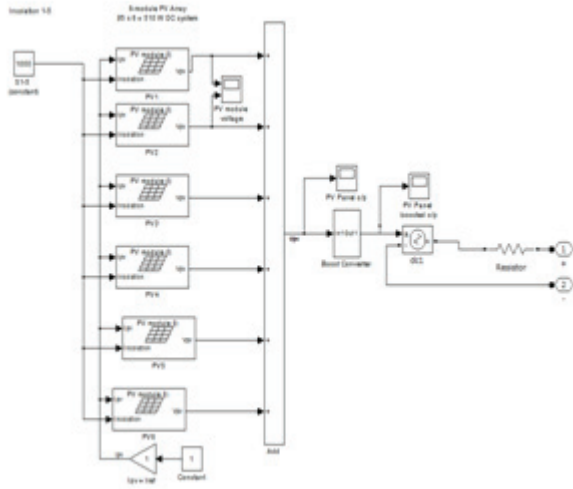
Fig. 11 Simulation of PV Module at DC micro grid
