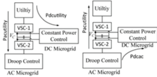
Fig. 8 Power flow schemes in Case 2
