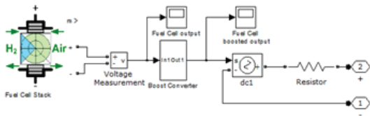
Fig. 12 Simulation of Fuel stack at DC micro grid
