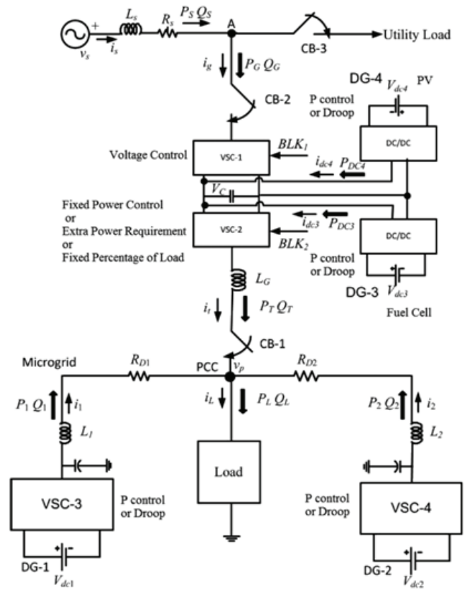
Fig. 1 System structure with AC/ DC micro grids
