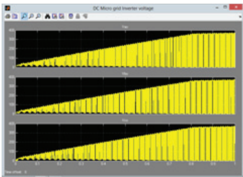
Fig. 18 Simulated output of VSC at DC end
