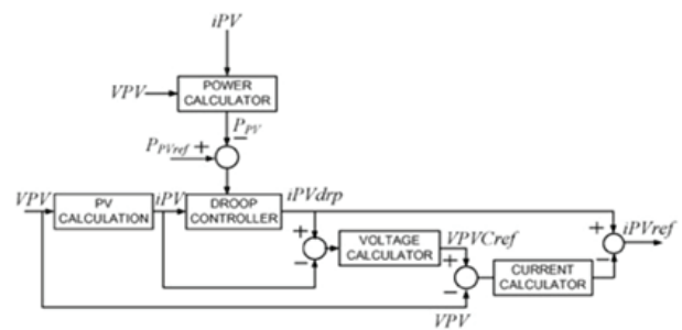
Fig. 4 Control scheme of the PV
