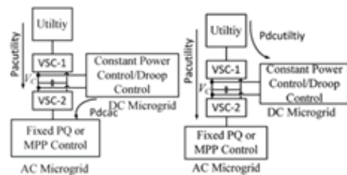
Fig. 7 Power flow schemes in Case 1
