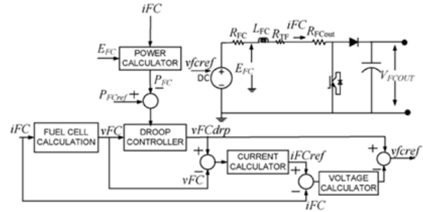
Fig. 3 Control scheme of the fuel cell
