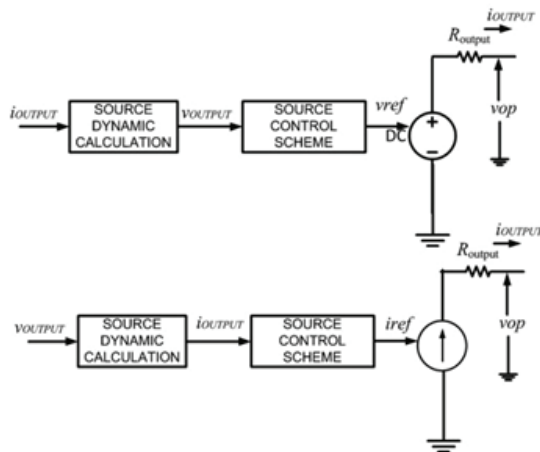
Fig. 2 Control schemes of the DC micro sources
