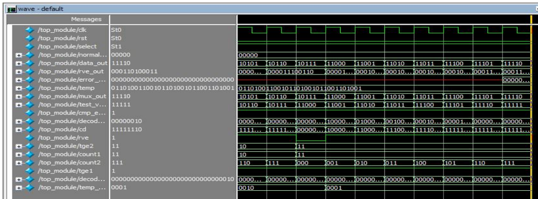
Fig.12 Simulation result of Modified SRAM-based BIST scheme in test mode.
