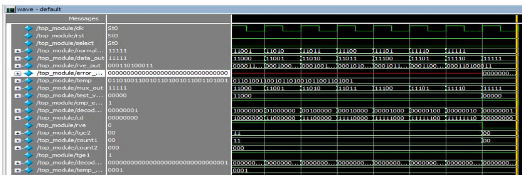
Fig.11 Simulation result of Modified SRAM-based BIST scheme in normal mode.
