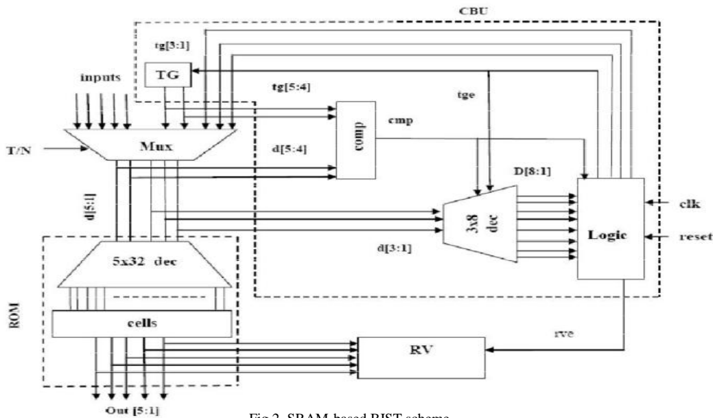
Fig.2 SRAM-based BIST scheme.
