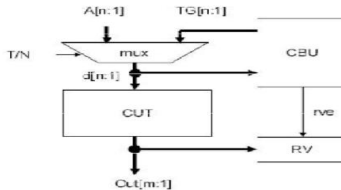
Fig.1 Input Vector Monitoring Concurrent BIST.
