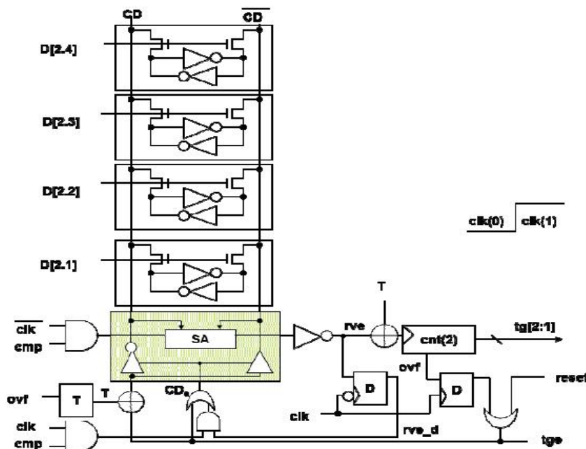
Fig.7 Logic Module.
