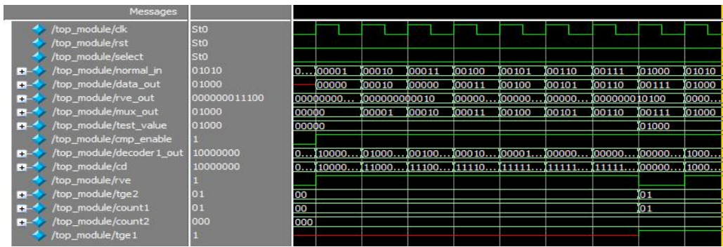
Fig.9 Simulation result of the SRAM-based BIST for ROM in Normal Mode.
