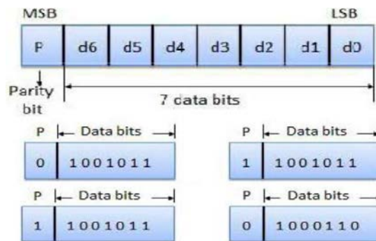
Fig.8 Even and Odd parity.
