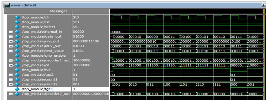
Fig.10 Simulation result of SRAM-based BIST scheme in test mode.
