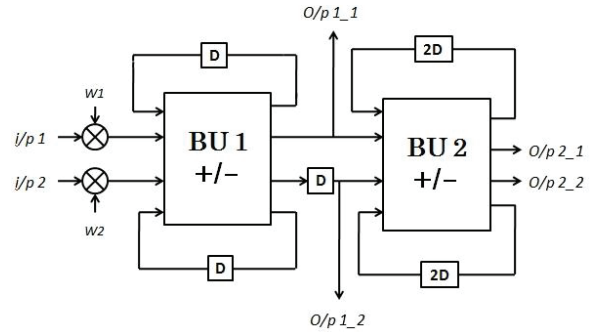
Fig 2 Reduced point FFT Processor Architecture
