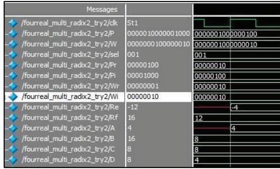
Fig. 10 Simulation Output of Complex Multiplier Unit
