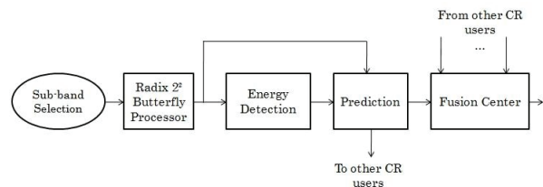
Fig 5 Co-operative Spectrum Sensing Architecture
