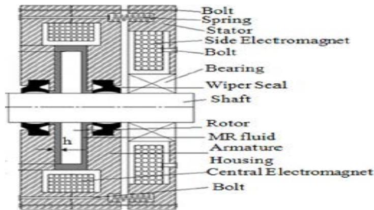
Fig. 5 Shear Plus Squeeze Mode based Magnetorheological Brake
