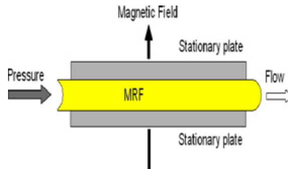
Fig. 1 Valve mode [3]
