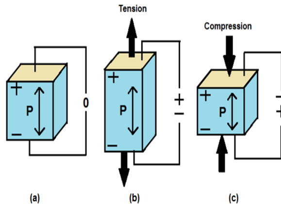
Fig.2. Piezoelectric effect
