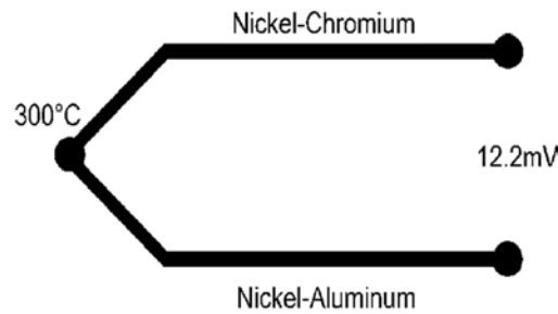
Fig.3 Thermocouple
