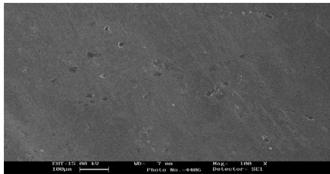
Fig.3 (b) SEM Micrograph of worn surface of AISI D3 steel pin at speed 1.67 m/s
