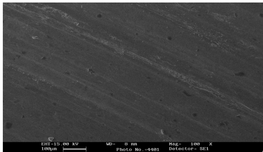
Fig.3 (a) SEM Micrograph of worn surface of AISI D3 steel pin at speed 1.15 m/s
