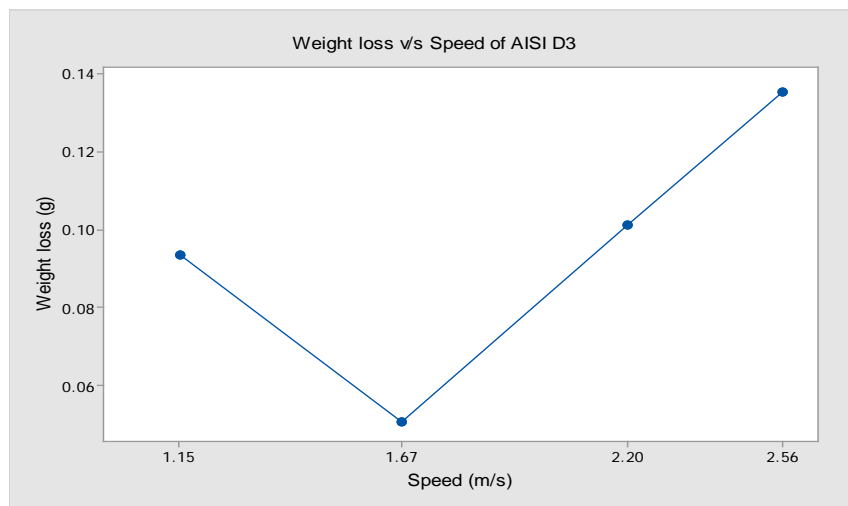
Fig.1 Weight loss vs speed of AISI D3
