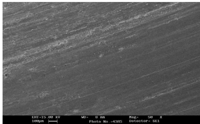
Fig.3 (c) SEM Micrograph of worn surface of AISI D3 steel pin at speed 2.56 m/s
