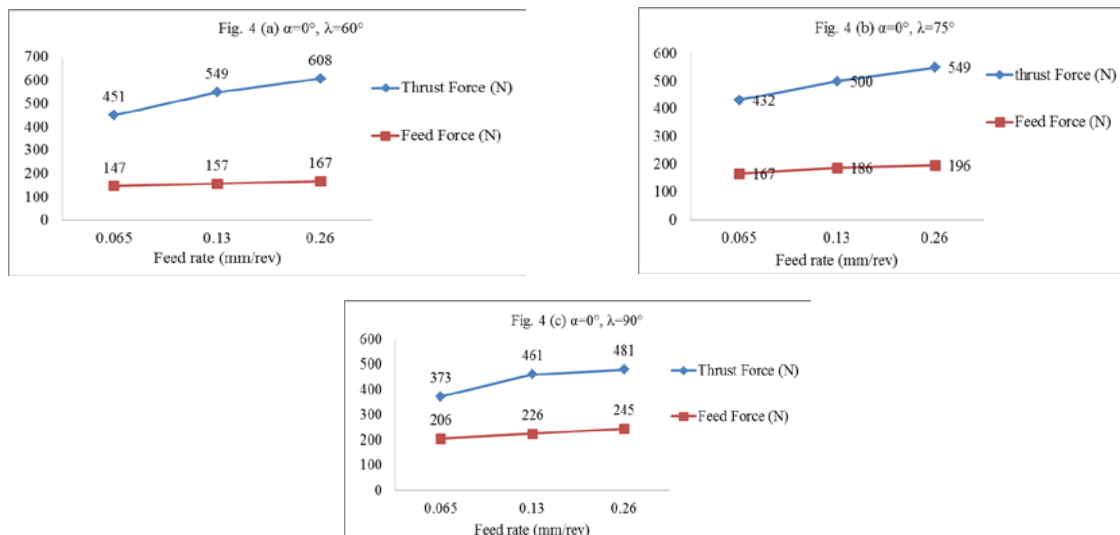
Fig.4 Cutting forces and tool tip temperature change due to the feed rate in different approaching angles
