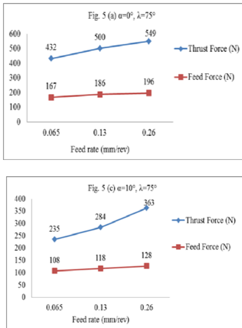
Fig.5 Cutting forces and tool tip temperature change due to the feed rate in different rake angle
