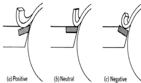
Fig.1 Types of rake angle
