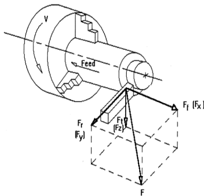
Fig.2 Components of cutting forces
