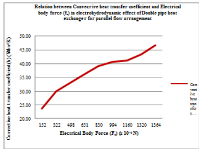
Fig. 3 Variation of electrical body force (fe) v/s convective heat transfer (h)
