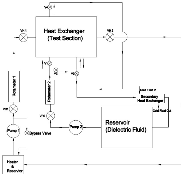
Fig. 1 Block diagram of the experimental setup (Not to scale)
