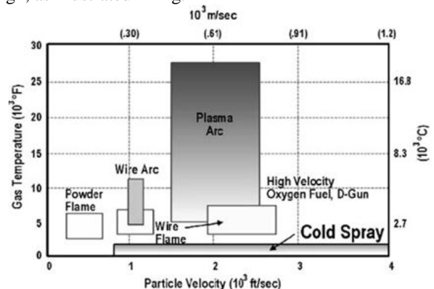
Fig. 1 Process temperatures and particle velocities of various coating processes [6]
