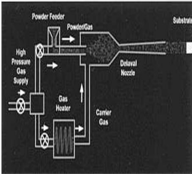
Fig. 2 Setup of cold spray coating
