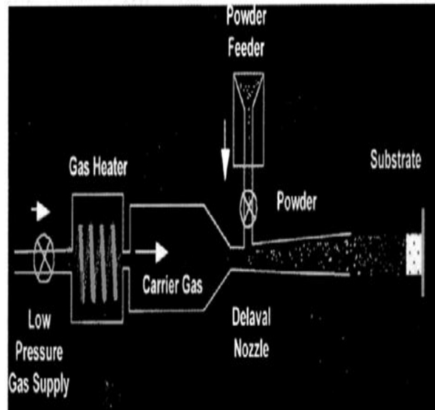
Fig.4 Schematic diagram of a variant of the cold spray process, where the powder is injected downstream in the DeLaval nozzle [12].
