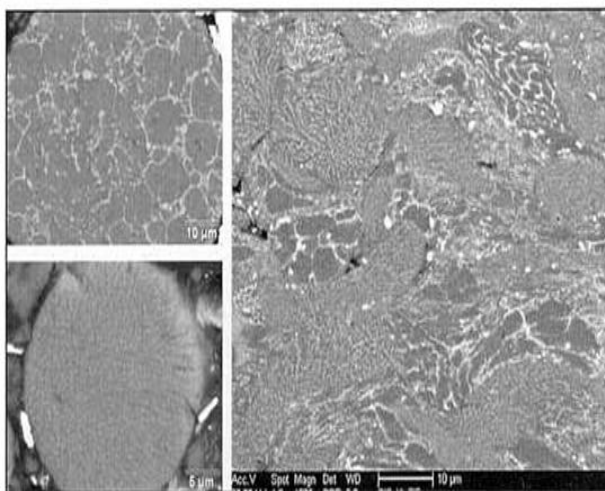
Fig. 3 Left: Particles of AA2618 aluminium alloy with equiaxed (top left) and columnar (bottom left) grain structures. Right: Cold spray deposit produced with a blend of these two powders showing the preservation of the original grain structure for each of the powder constituents (Ref. 5) (Photo courtesy of the University of Ottawa, Canada.)
