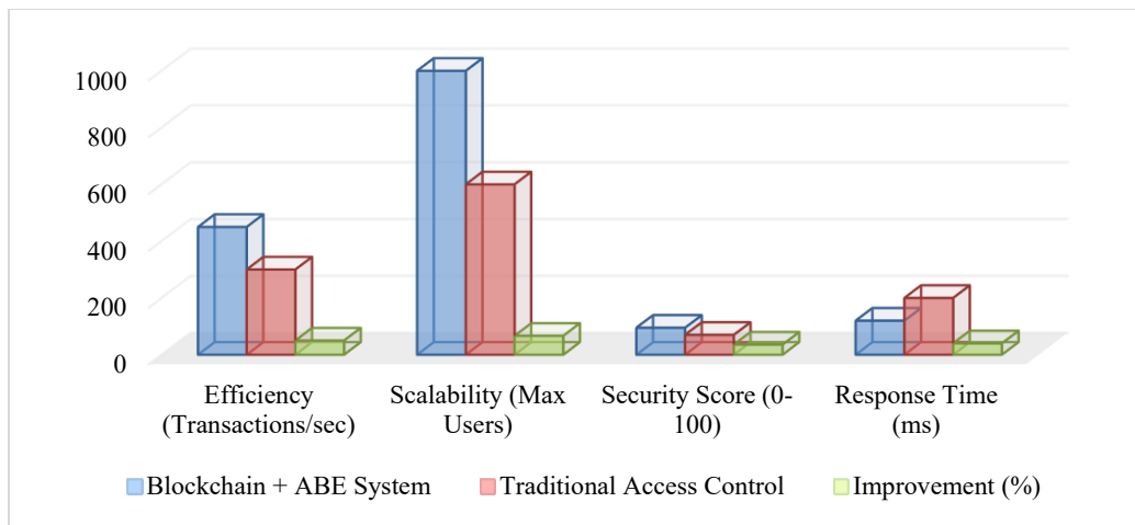
Fig. 2 Performance and Security Comparison: Blockchain-Based ABE System vs Traditional Access Control
